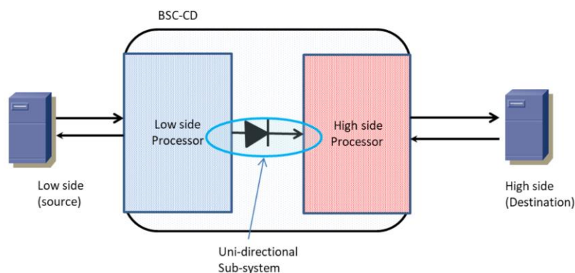
Figure 1: TOE Architecture
